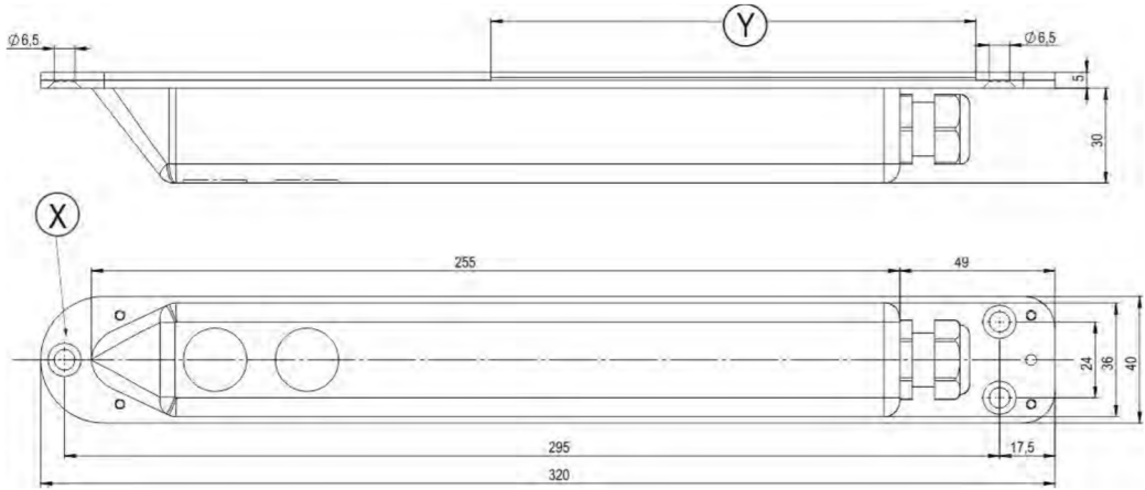
Fig. 4-21 Dimensions sensor OCL
