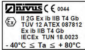
Fig. 4-30 Ex label for sensor CSM
