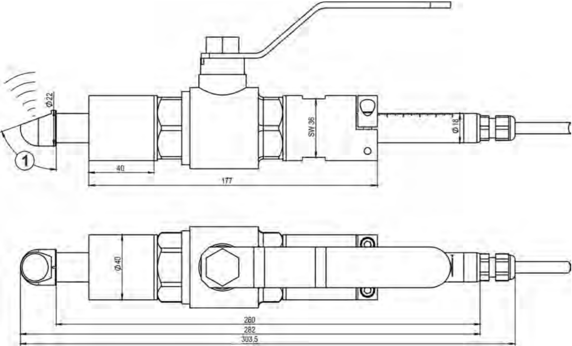
Fig. 4-7 Basic construction sensor CSM-V100R
