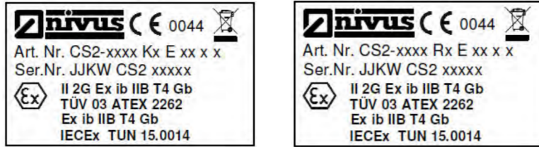
Fig. 4-41 Nameplates sensor CS2
