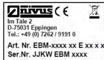
Fig. 4-33 Nameplates Electronic Box, type EBM
