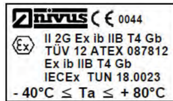
Fig. 4-32 Ex nameplate for pipe sensor, type CSM-V100R
