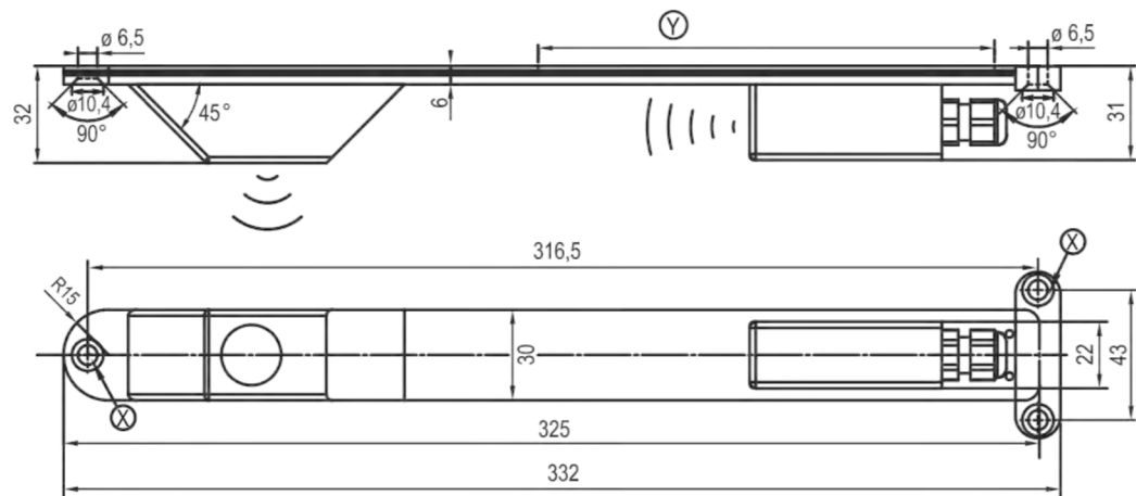
Fig. 4-9 Basic construction sensor DSM
