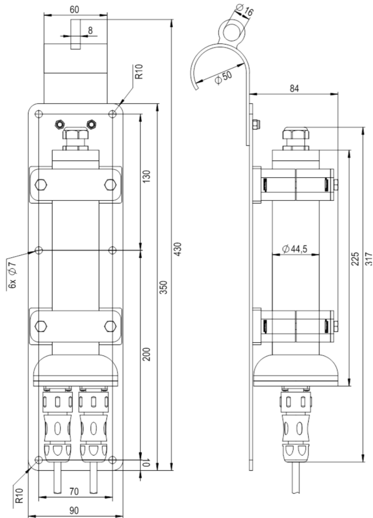
Fig. 4-12 Dimensions Electronic Box EBM
