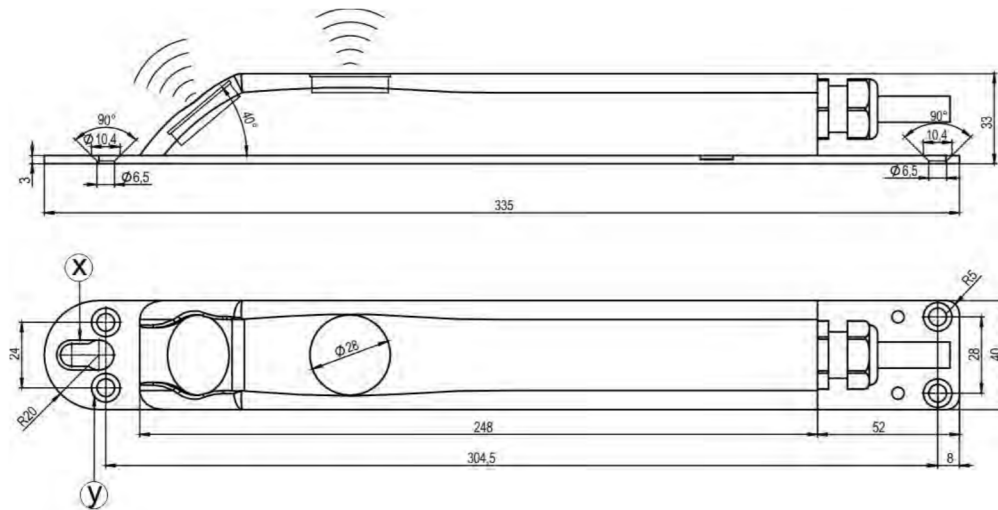
Fig. 4-26 Basic construction sensor CSP
