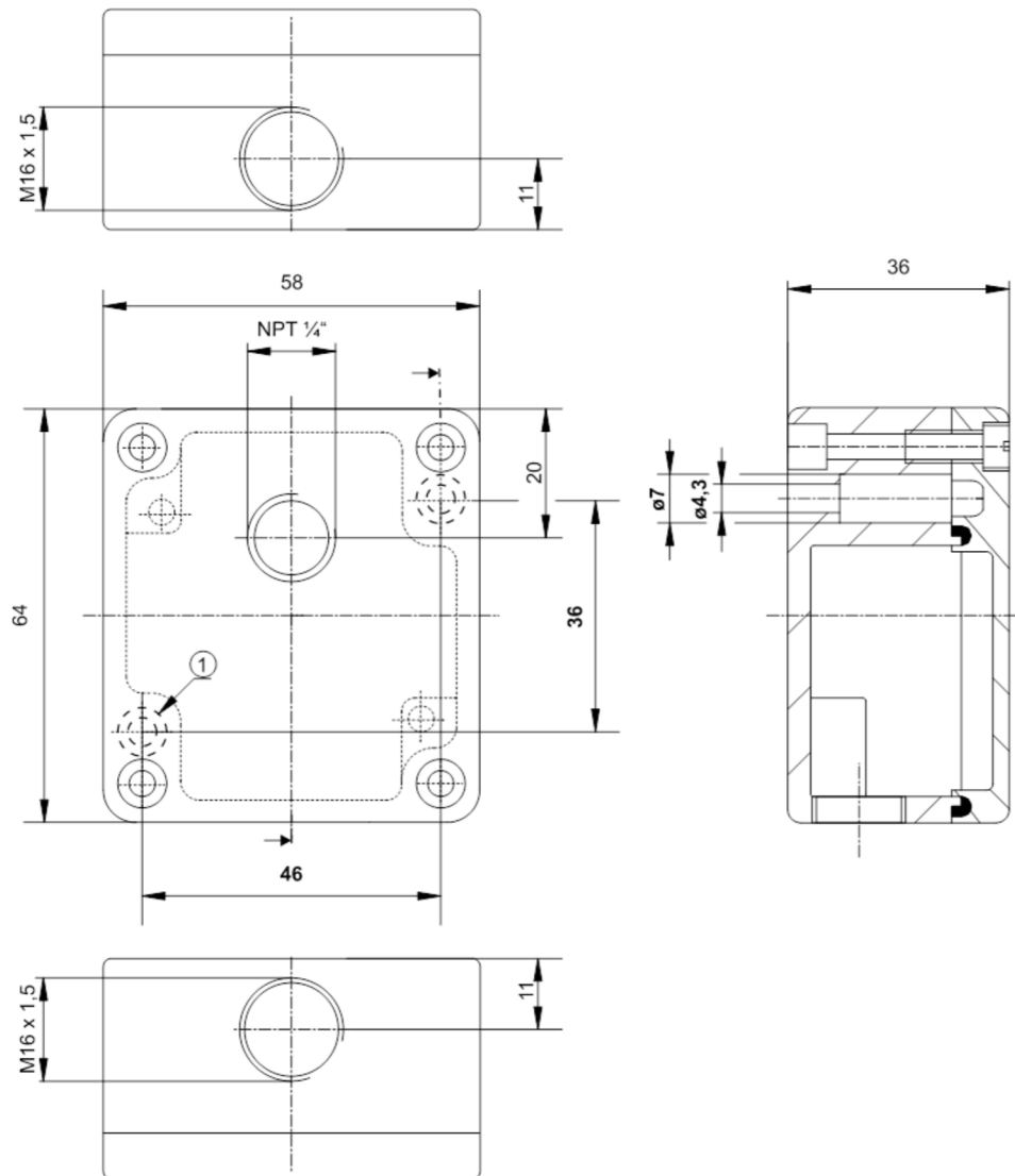
Fig. 5-14 Connection box dimensions
