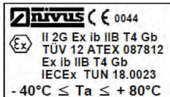
Fig. 4-38 Ex nameplates for sensor CSP
