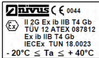
Fig. 4-34 Ex nameplates Electronic Box, type EBM
