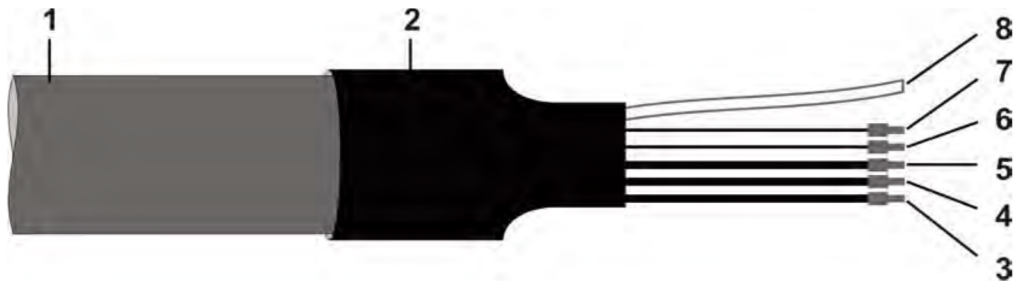
Fig. 5-6 Cable end configuration; sensors POA and CS2 without press. meas. cell
