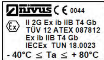
Fig. 4-36 Ex label for sensor DSM
