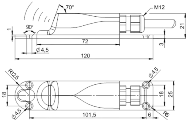
Fig. 4-4 Dimensions sensor CSM-V100K
